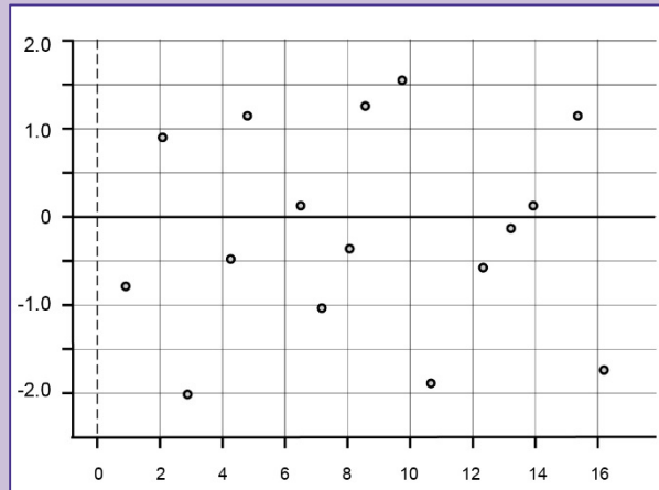
residual plot
